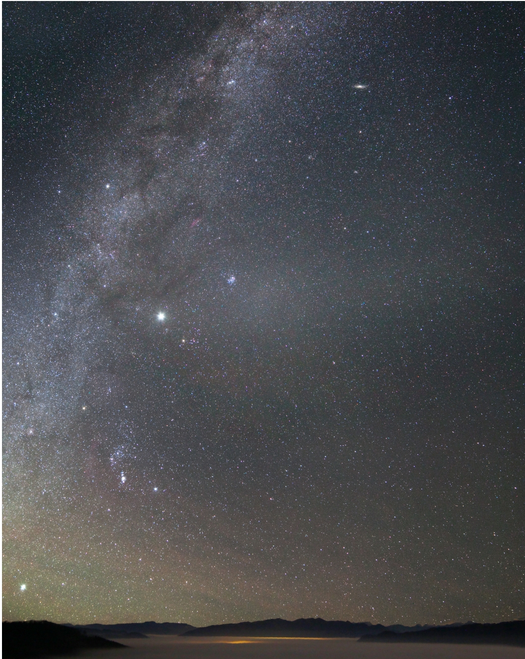
Fig. 12.7: Gegenschein in the zodiacal band (centre) in the Eastern Alpine Starlight Reserve above the Kalkalpen National park as seen from the “Hohe Dirn” (1000m). The Milky Way is rising on the left. Photograph: R. Dobsberger, Sternfreunde Steyr
